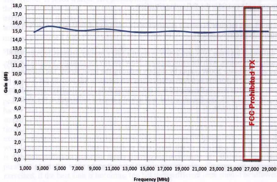
KL505 Gain vs Frequency
